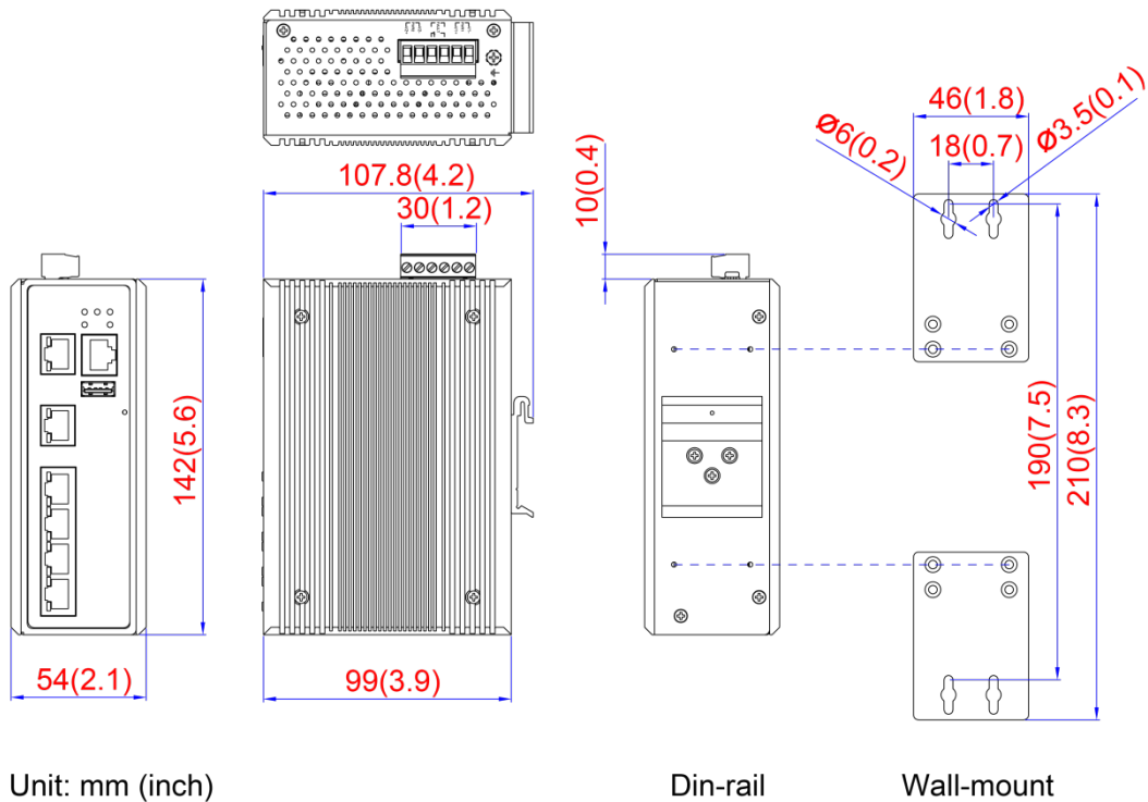
Figure 2.1: Physical Dimensions
