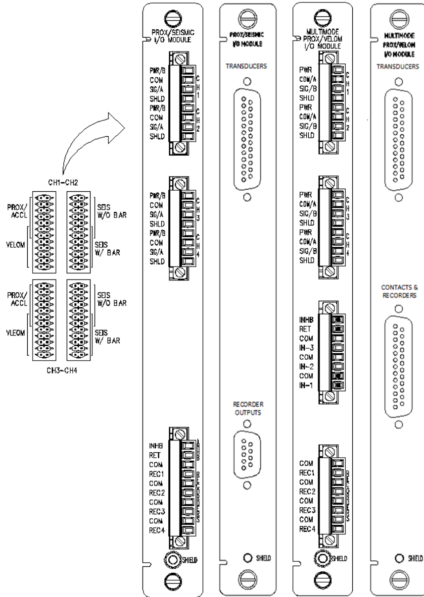
Figure 2: Side View of I/O Modules
